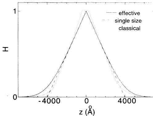
FIG. 8. Comparison of the z variations of the single domain finite-size factor (dashed line) in Eq. (68), the classical (Gaussian) finite-size factor (dotted line) in Eq. (17), and our effective finite-size factor H_{eff}(z) (solid line) from Eq. (82) for L_0 = 4000 \text{ \AA} , \sigma_L = 1200 \text{ \AA} .
